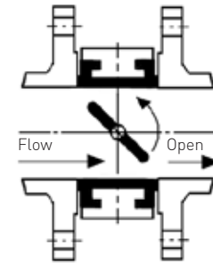
Preferred mounting
